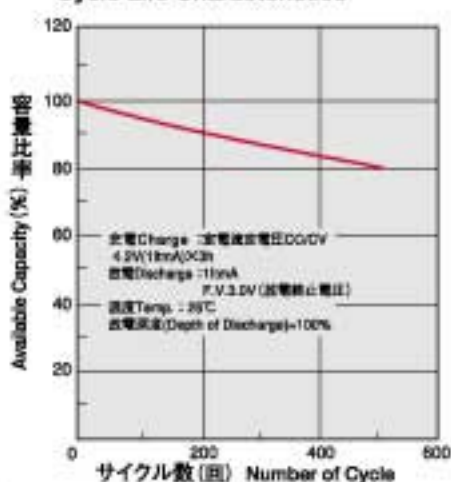
Cycle Life Characteristics
